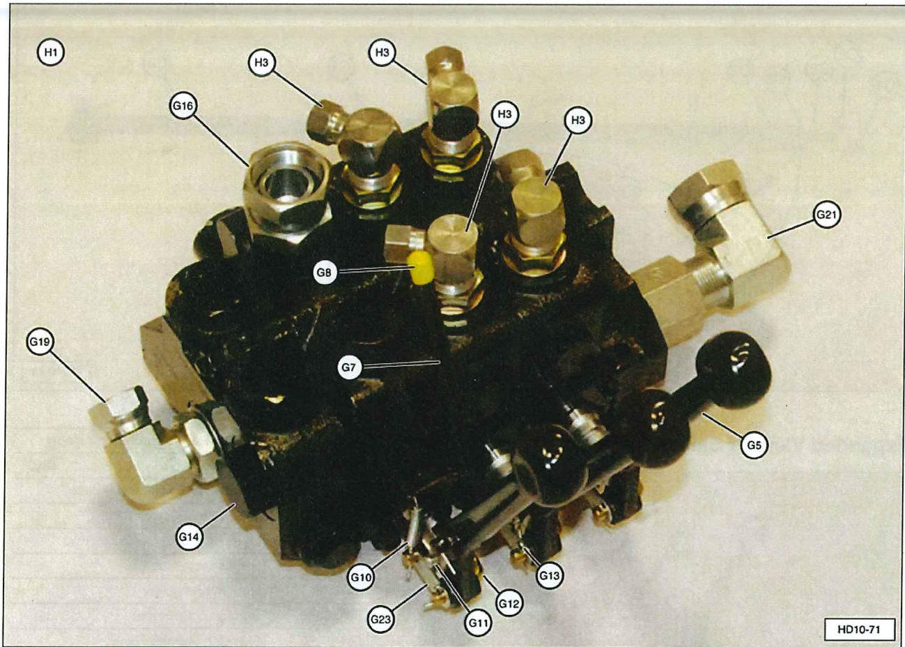
HD-10-H Service Parts - Triple Control Lever Valve
