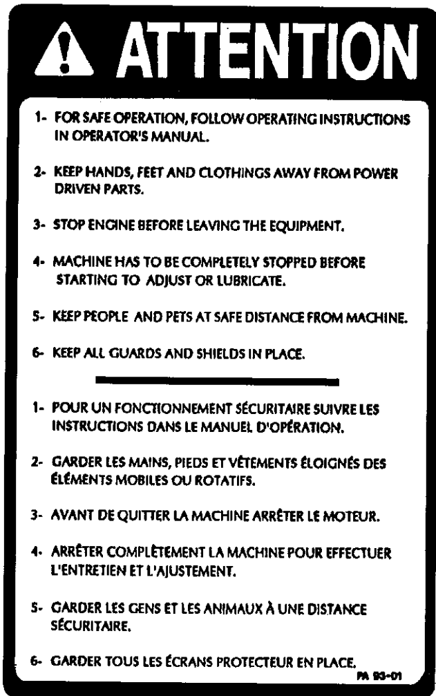
Figure 2 Decal A
