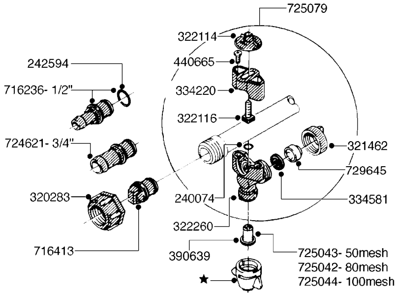
SINGLE NOZZLE BODY
