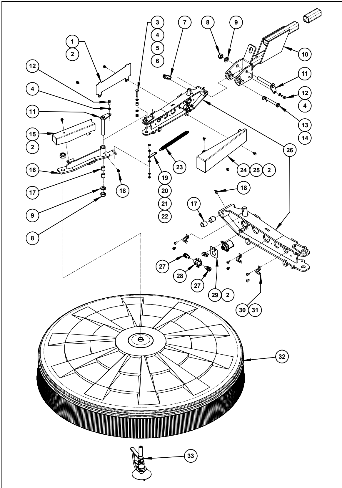
Figure 5 – Spraydome 1200 CDA Outrigger Assembly
