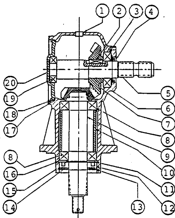
BOITE D'ENGRENAGE LF-135A No. 20411 GEAR BOX LF-135A
