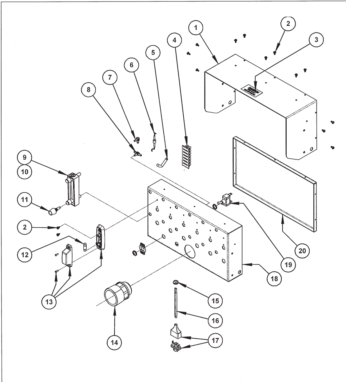
Figure 12 – Controller, Lamp Type, 6-Way
