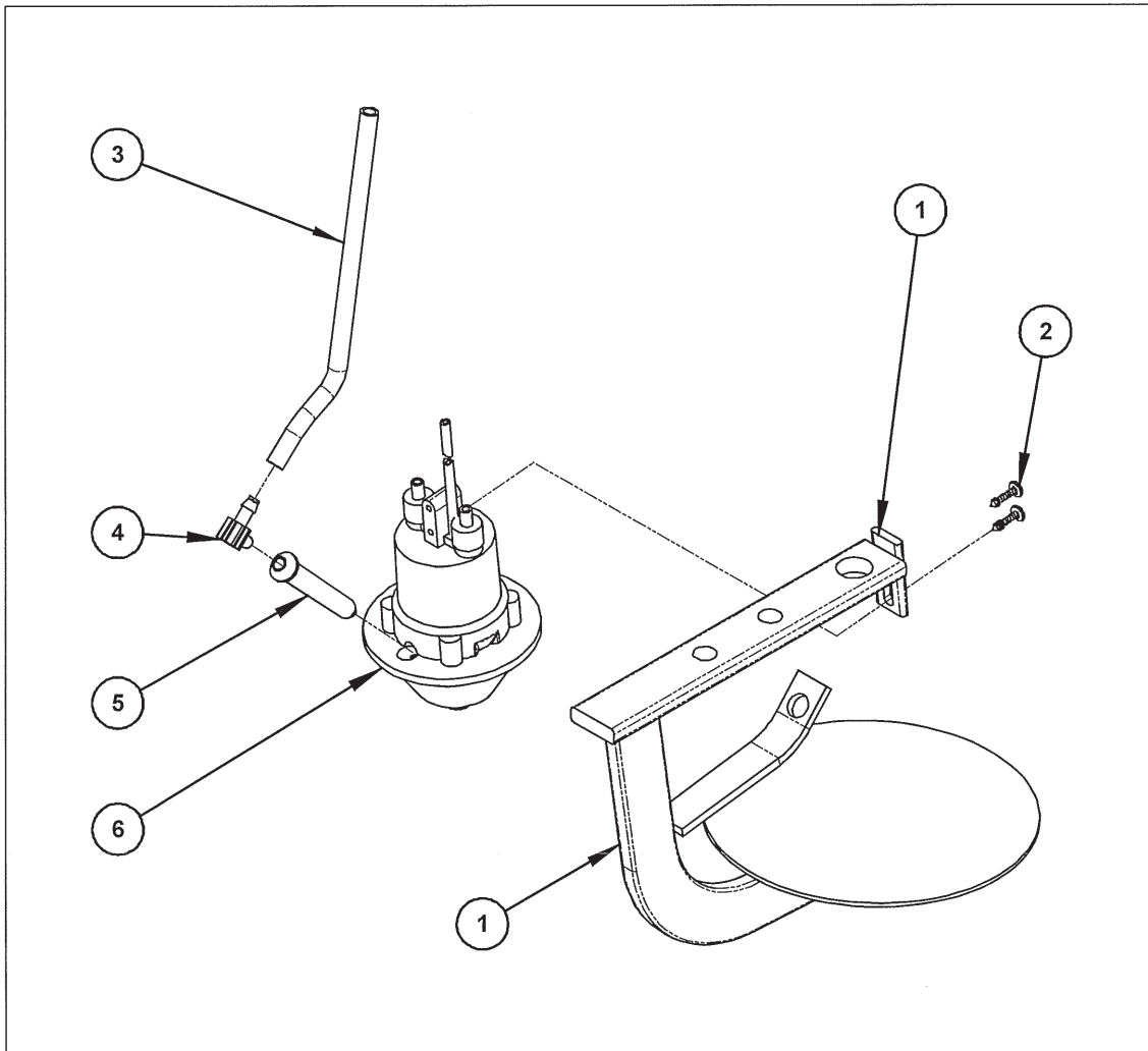
Figure 10 – Head Assembly Adjustable Spraydomey
