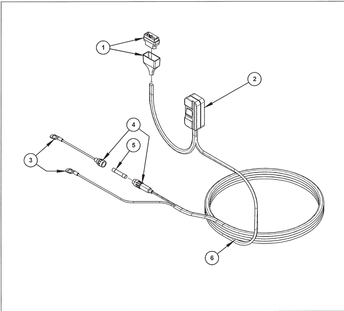
Figure 13 – Power Wire Assembly
