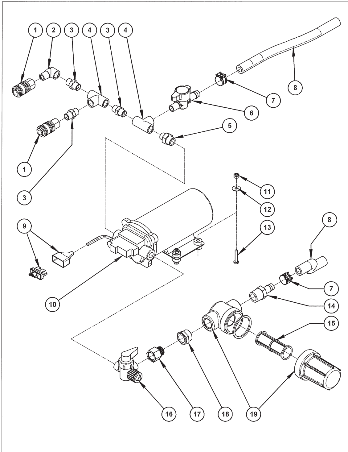
Figure 7 – Pump System Components
