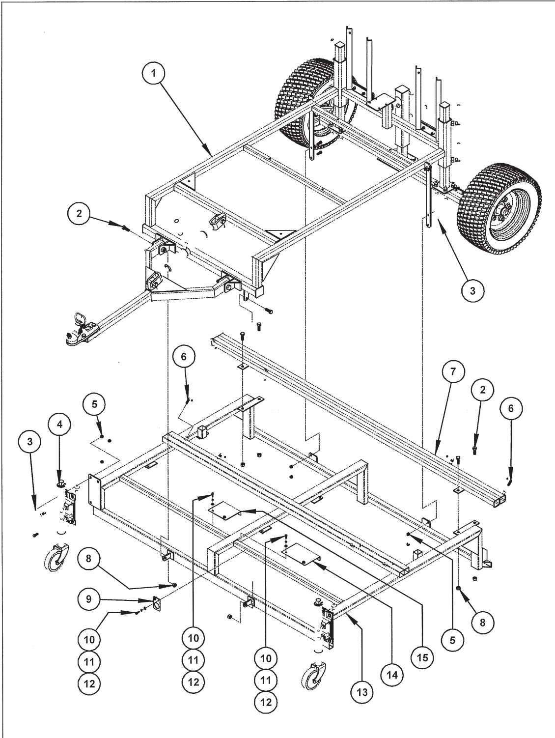
Figure 3 – Chassis Components
