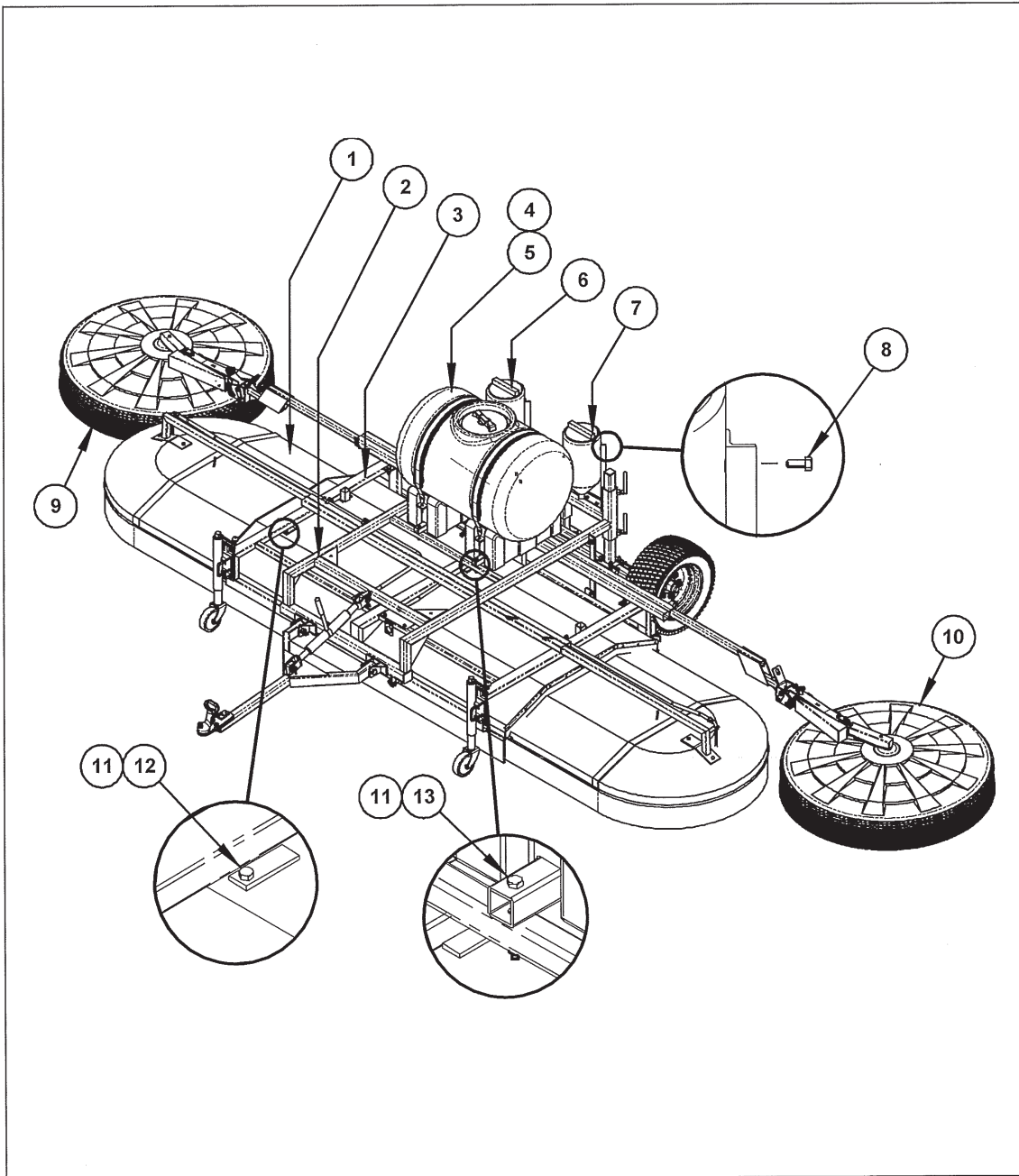
Figure 1 – 3049 CDA Major Assemblies and Fixings
