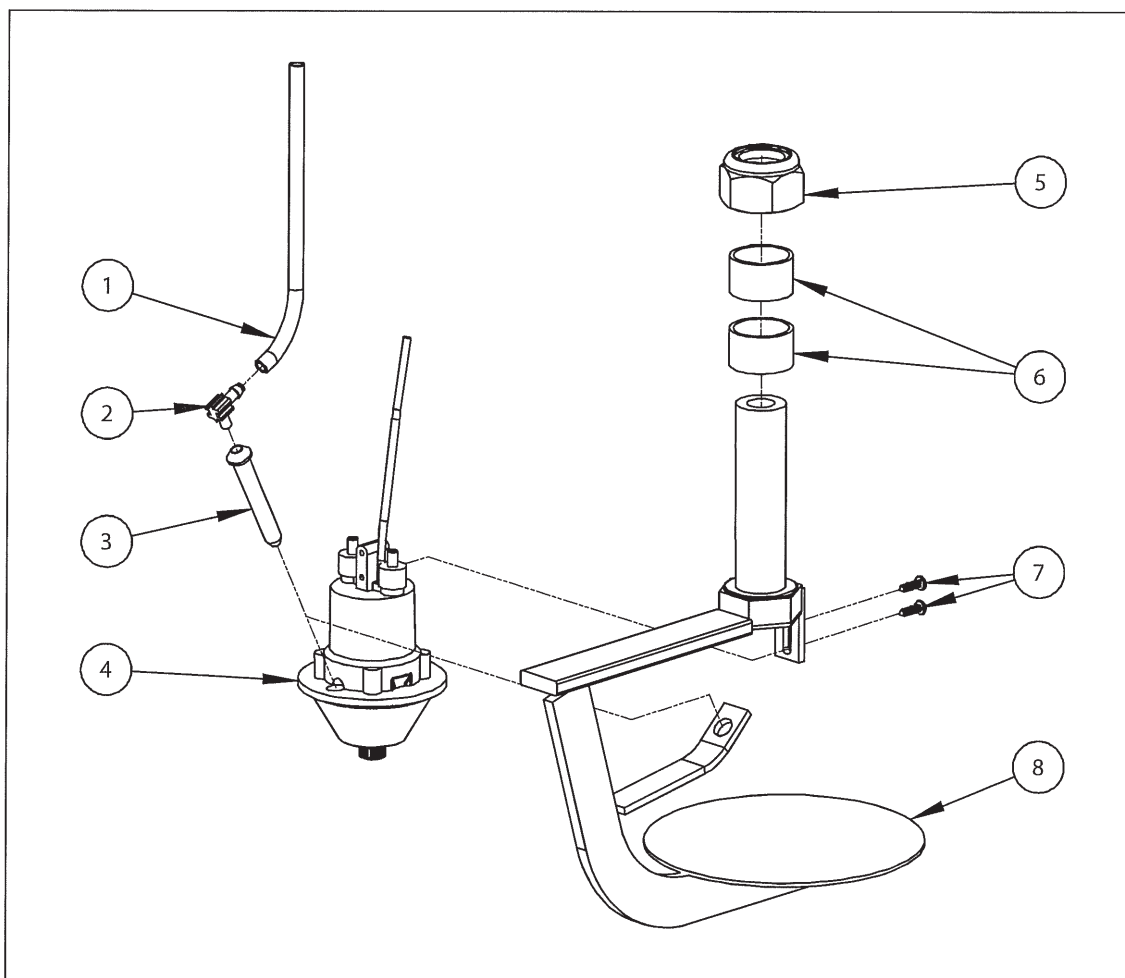
Figure 9 – 1000/1200 CDA Head Assembly
