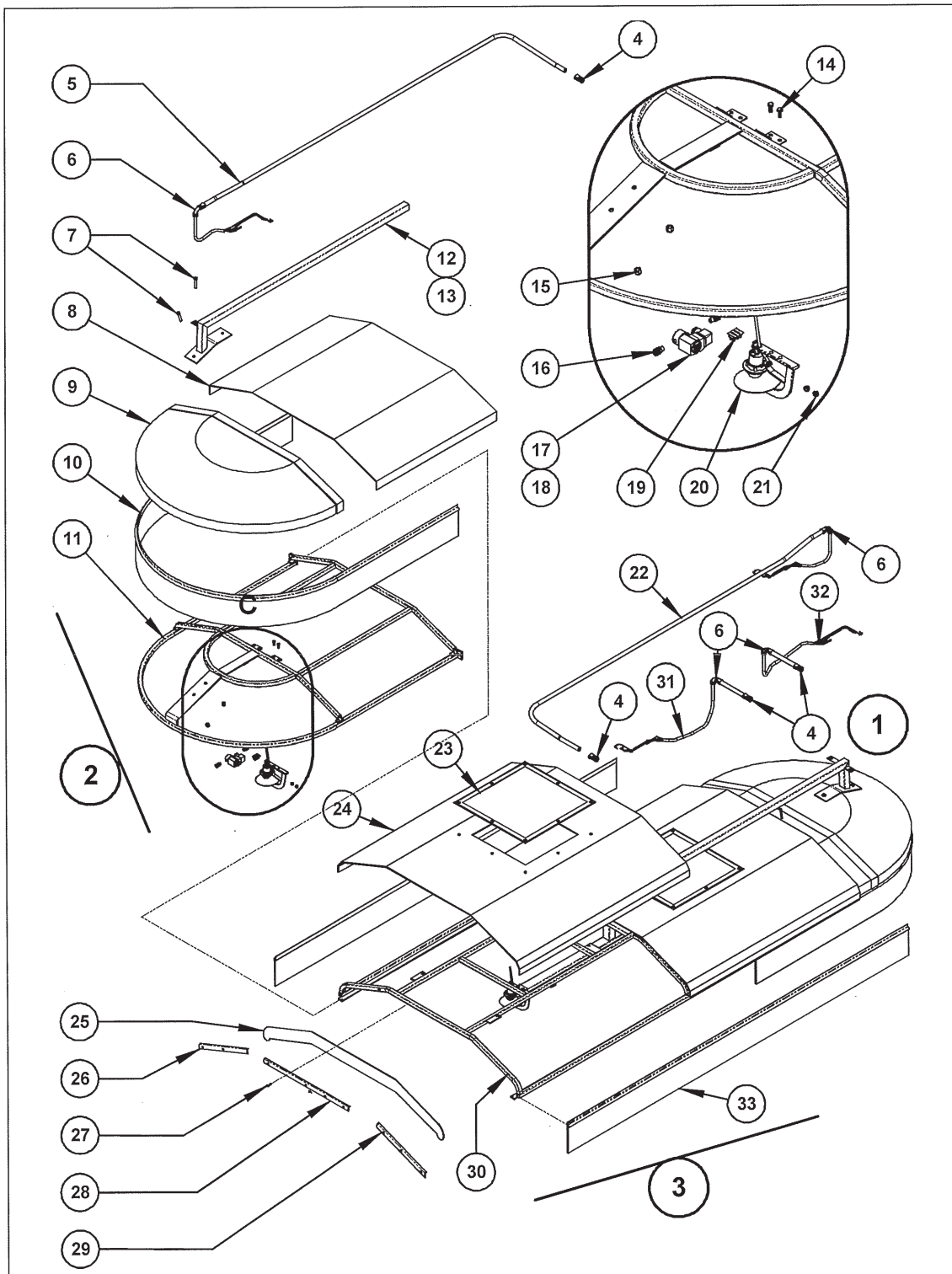
Figure 2 – Shield Assembly
