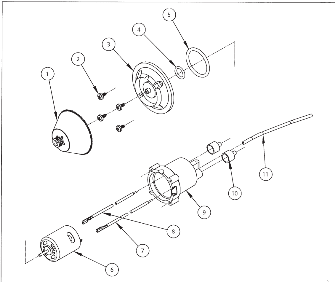
Figure 11 – CDA Head Assembly with Atomiser Disc - Ulva+ (ZD004)
