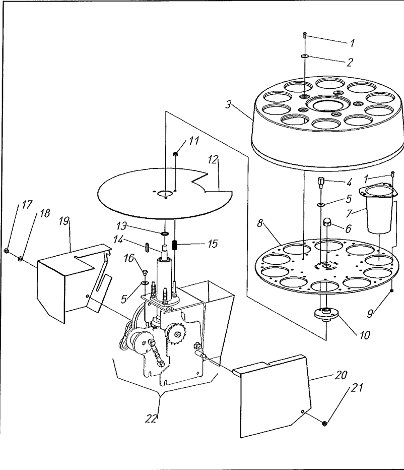
TAV.06 DISTRIBUTOR TRIUM 10 HOLE
