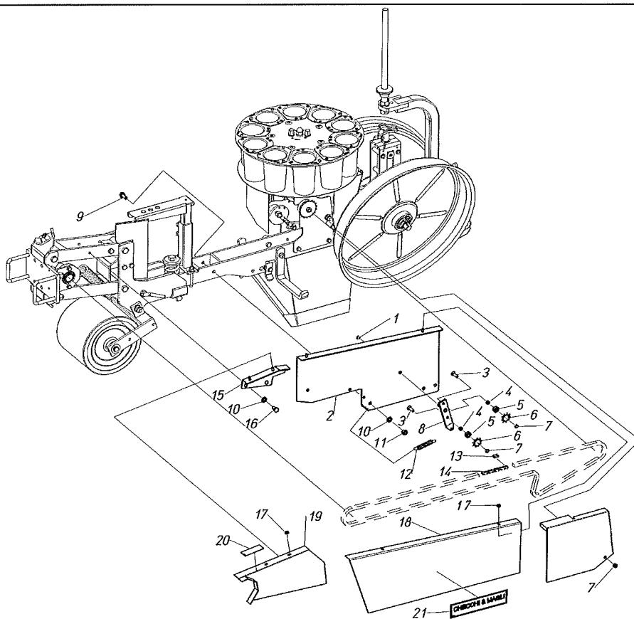
TAV.09 - COVERS AND CHAIN FOR DISTRI TRIUM
